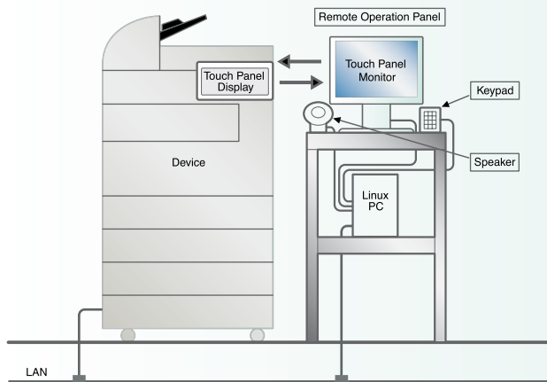
Using the Remote Operation Panel requires a Linux PC connected to a LAN, a keypad, touch panel monitor, and a speaker.
